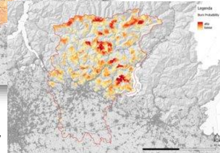
Burn Probability
